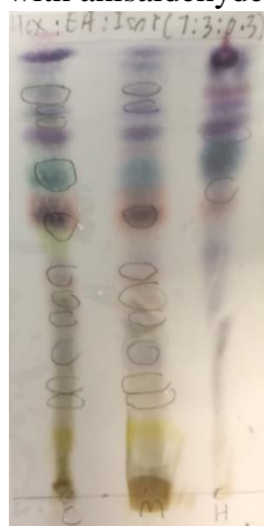
Figure 2. Chromatographic profile of P. canescens extract of mobile phase Hex: EA: IsoP (7:4:0.3). The left side of the plate is the chloroform extract. The middle part is the methanol extract, while the right side is the hexane extract.
